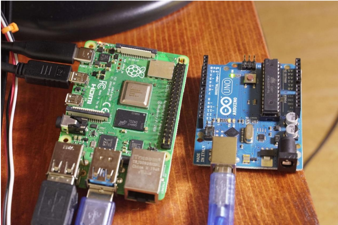
Fig.4.4 Serial Communication
